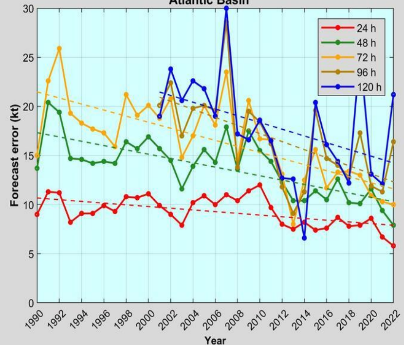
NHC Official Intensity Error Trend Atlantic Basin
