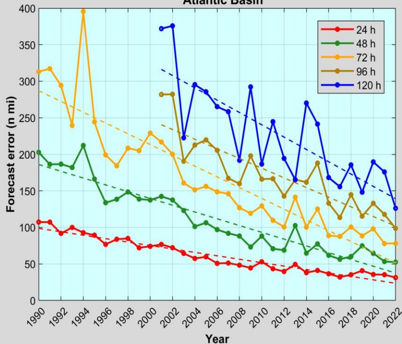
NHC Official Track Error Trend Atlantic Basin
